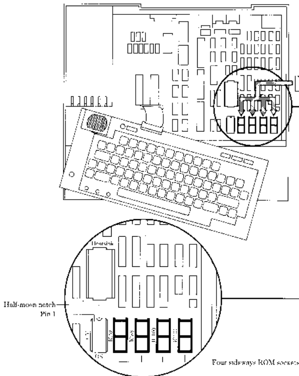
Figure 5 Inserting the Hi-BASIC ROM
